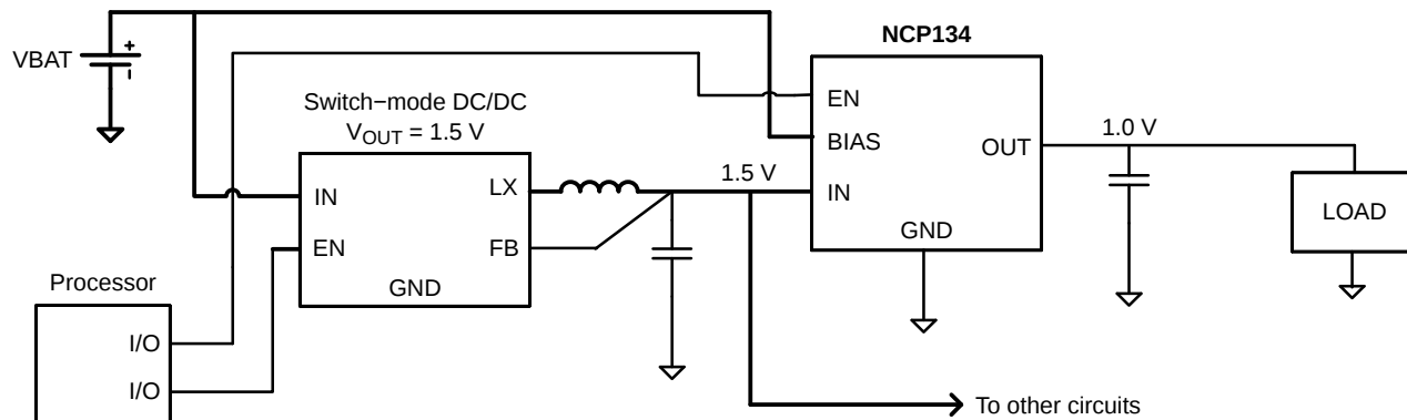
Figure 11. Typical Application: Low-Voltage DC/DC Post-Regulator with ON/OFF Functionality
